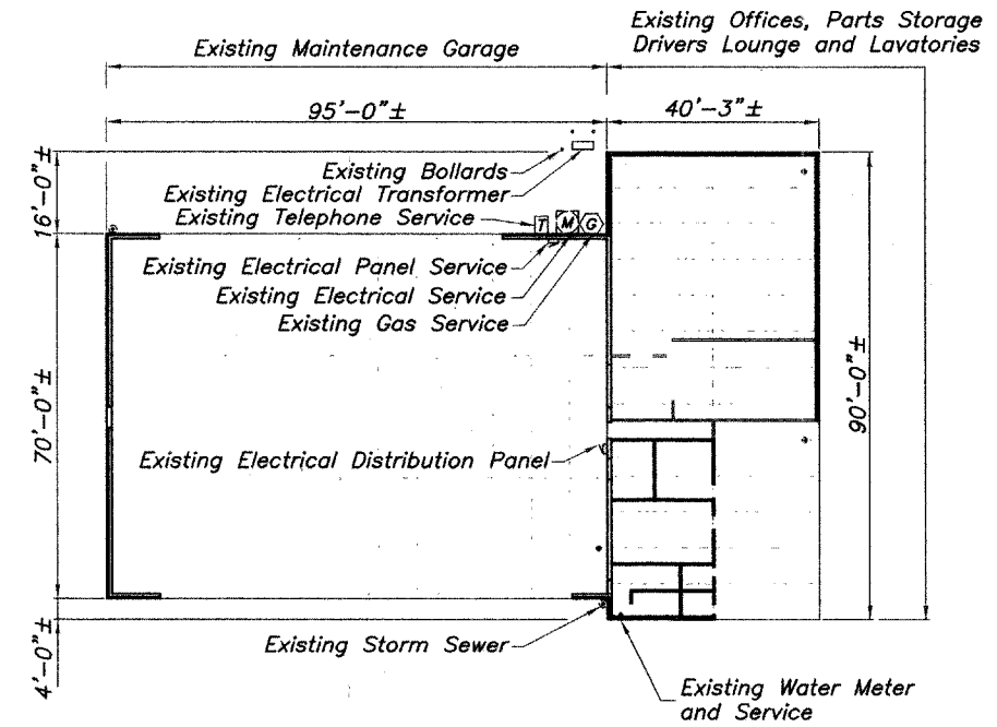
EXISTING BUILDING 205 - PLAN VIEW
