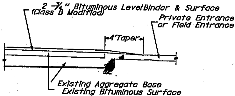
Entrance Taper Detail
