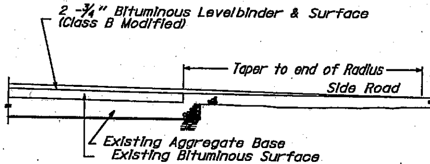
Side Road Taper Detail
