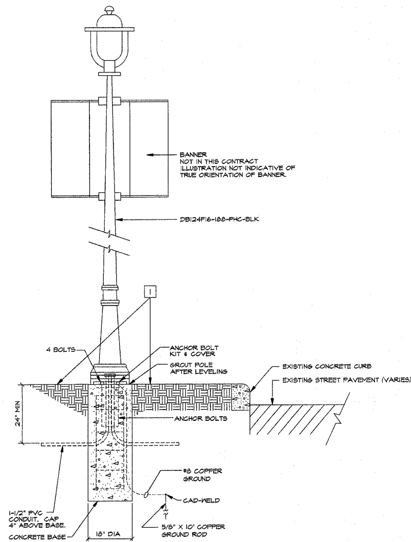
1 POLE & BASE DETAIL #1 NOT TO SCALE
