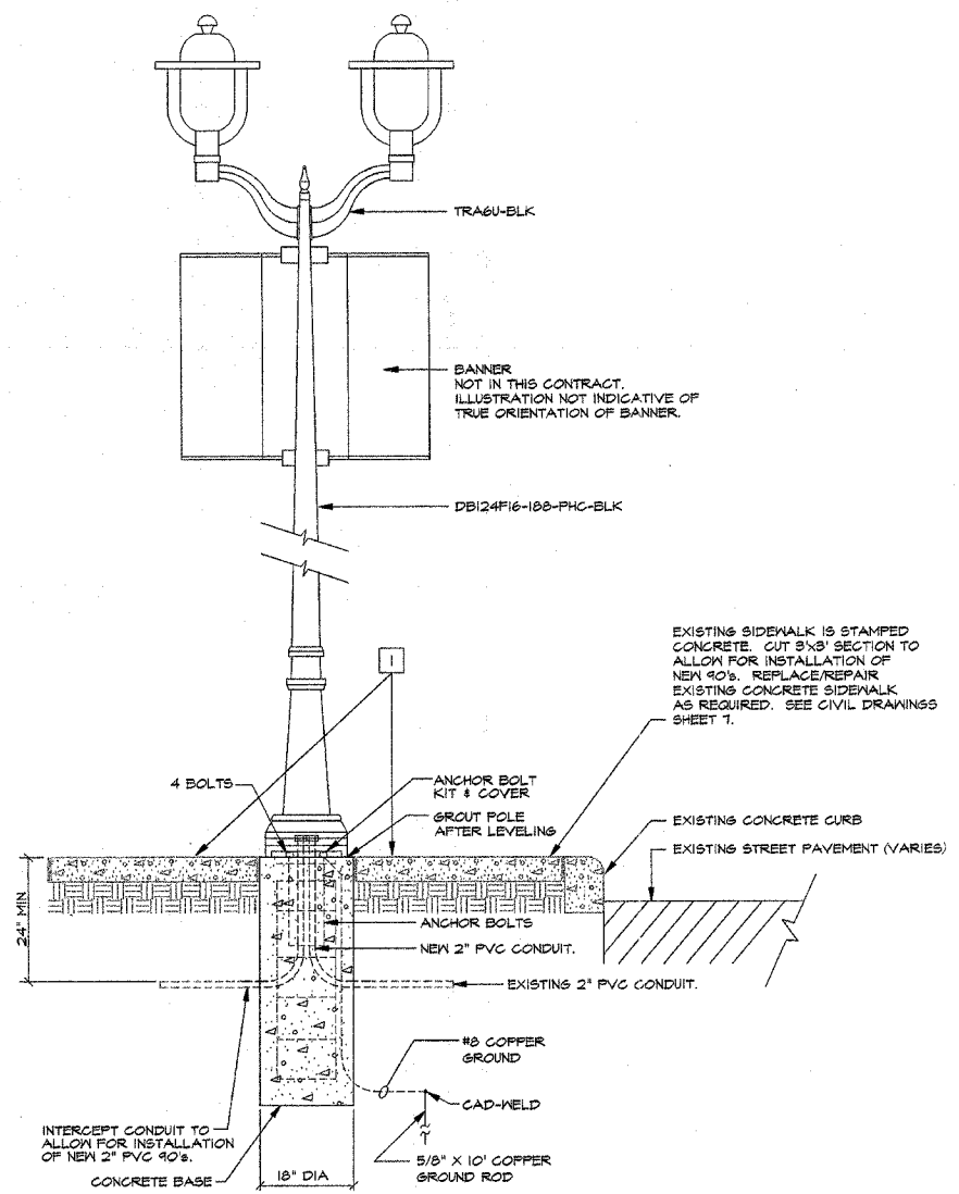
2 POLE & BASE DETAIL #2 NOT TO SCALE
