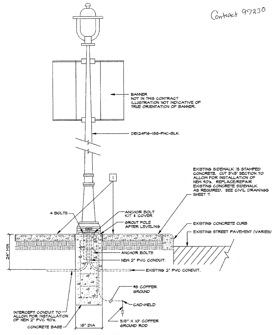
3 POLE & BASE DETAIL #3 NOT TO SCALE
