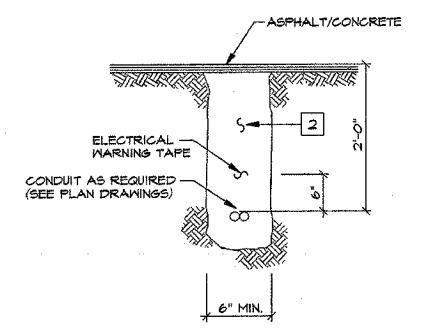
4 TRENCH DETAIL NOT TO SCALE
