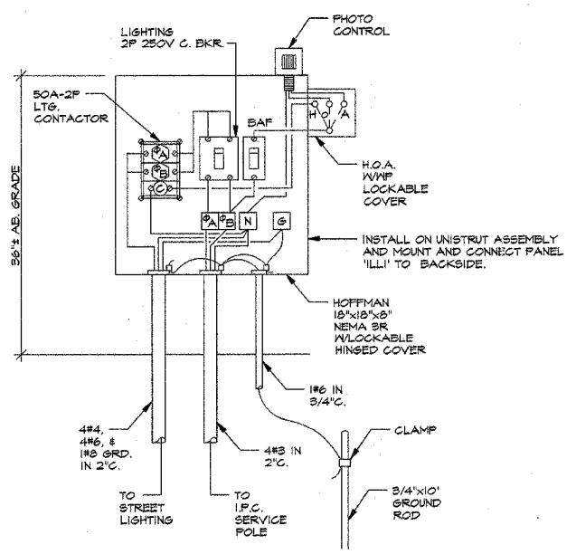
5 CONTROL DETAIL NOT TO SCALE
