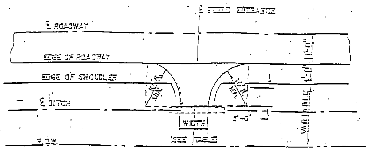
TYPICAL FIELD ENTRANCE DETAILS (12' MINIMUM WIDTH)
