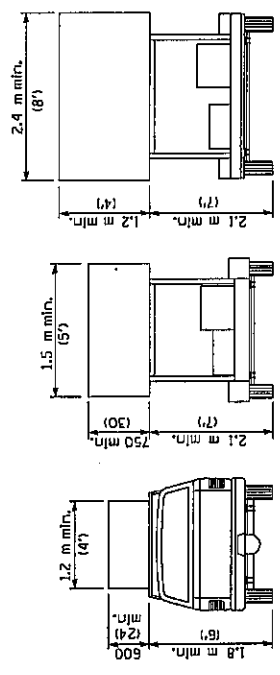
ARROW BOARDS
