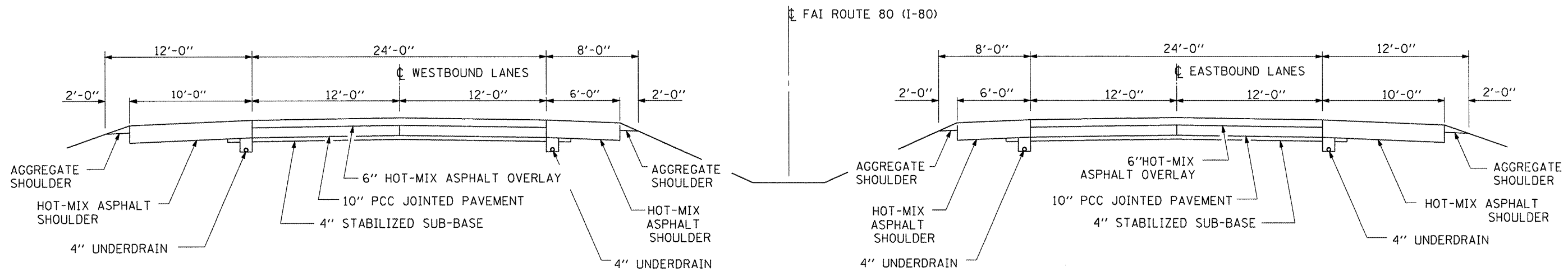
TYPICAL SECTION BUREAU COUNTY - FAI ROUTE 80 LOCATION 1 AND 2
