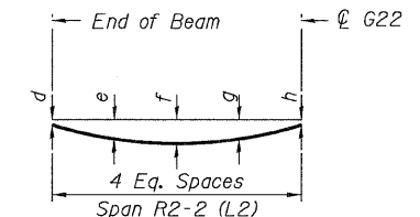
DEAD LOAD DEFLECTION DIAGRAM
