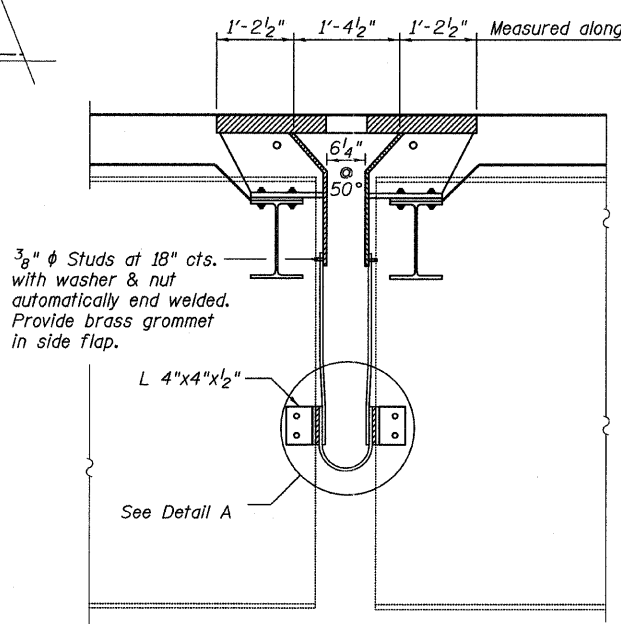
SECTION G-G THRU PIER 9 (Looking West)
