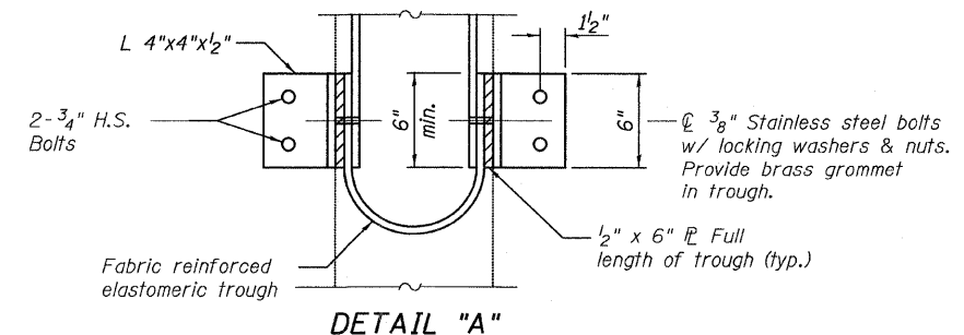
DETAIL "A"
