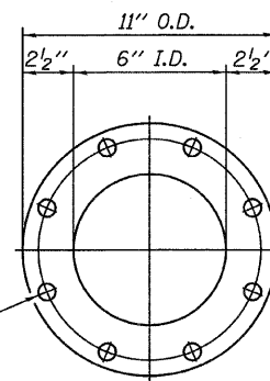
VIEW C-C
