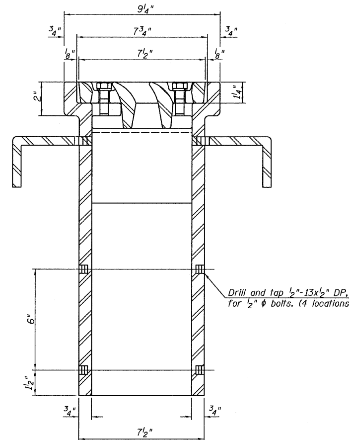
SECTION B-B
