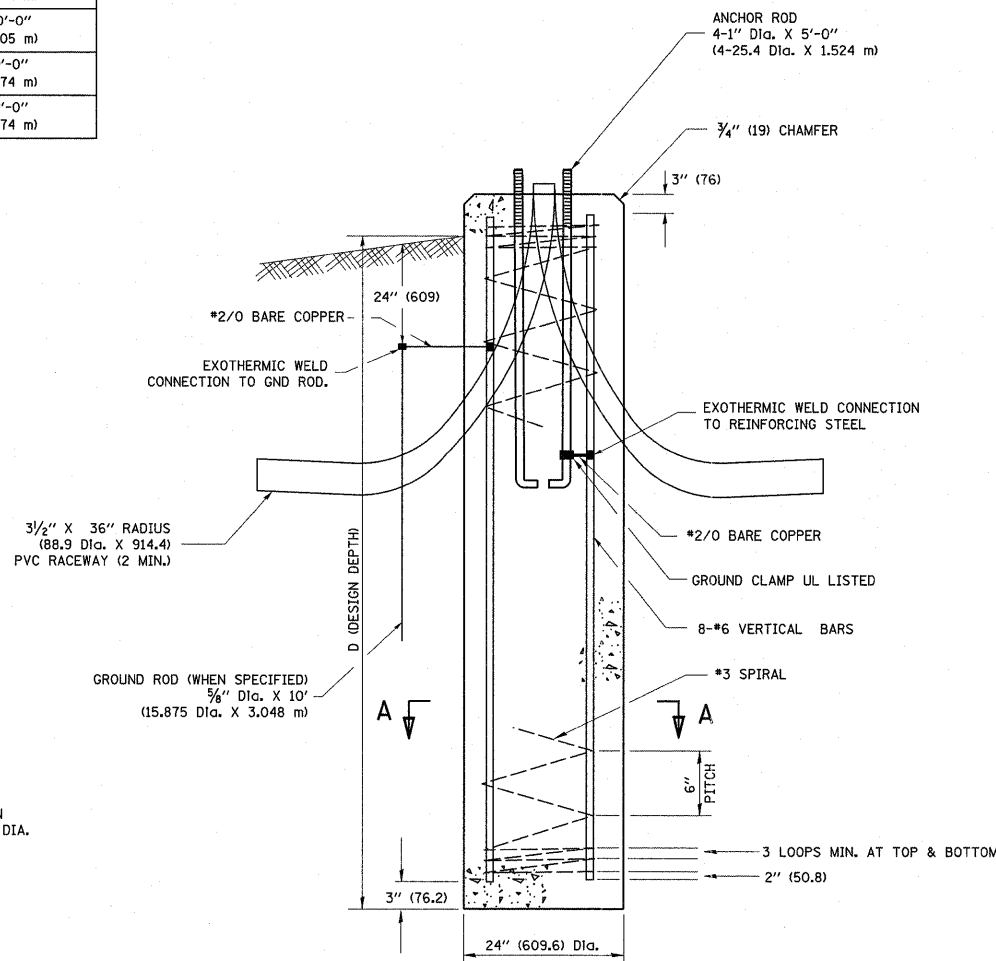
FOUNDATION DETAIL
