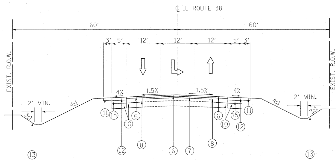
PROPOSED TYPICAL SECTION IL ROUTE 38
