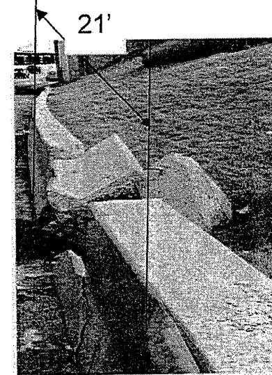
FULL DEPTH BARRIER REPAIR FOR MORE DETAILS SEE SHEET # 8
