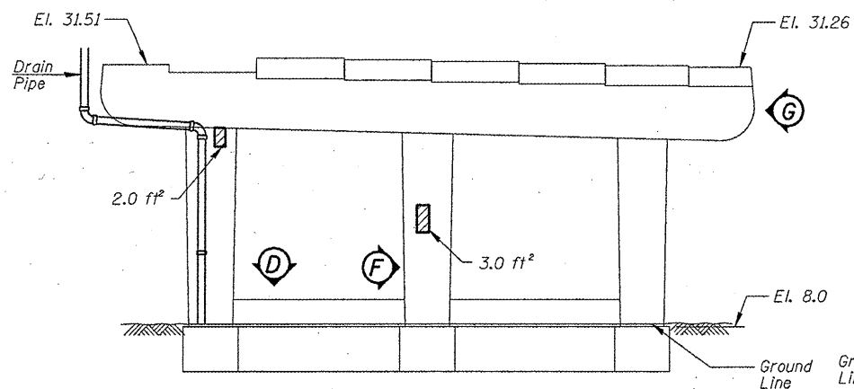
PIER D-10 - SOUTH ELEVATION (Looking North)
