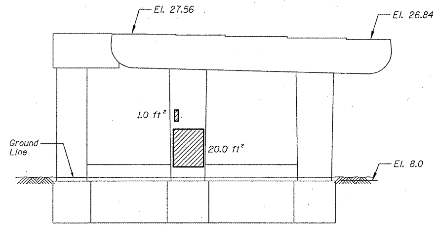
PIER D-11 - SOUTH ELEVATION (Looking North)
