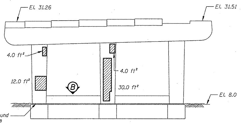
PIER D-10 - NORTH ELEVATION (Looking South)
