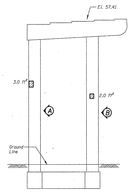
PIER C-2 - NORTH ELEVATION (Looking South)
