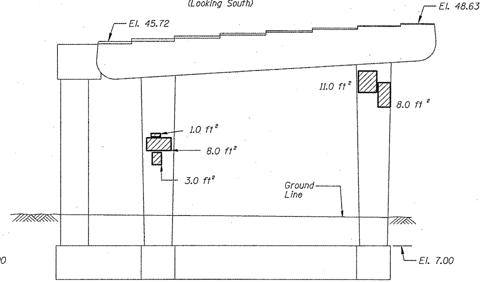
PIER A-8 - NORTH ELEVATION (Looking South)
