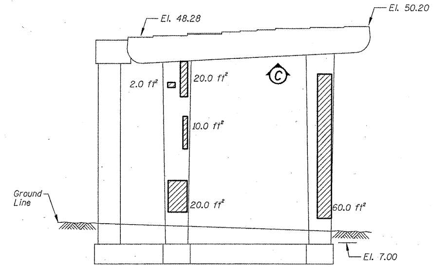
PIER A-7 - NORTH ELEVATION (Looking South)
