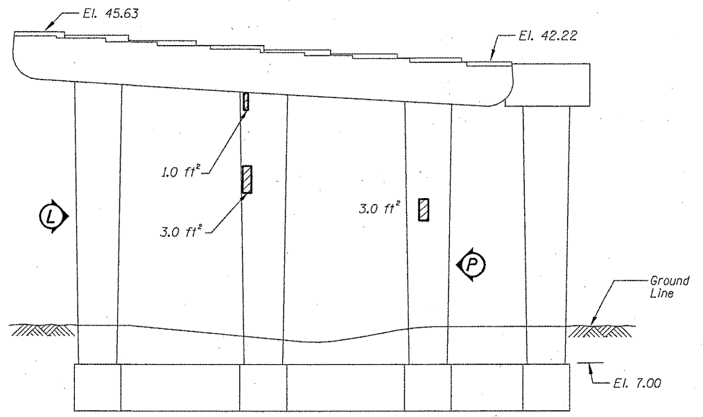
PIER A-9 - SOUTH ELEVATION (Looking North)
