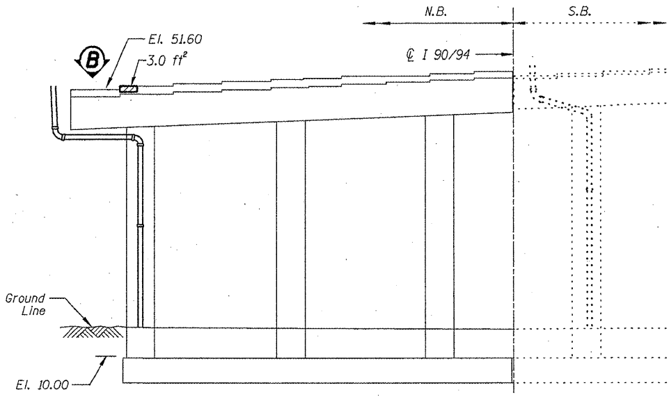
PIER 15 - NORTH ELEVATION (Looking South)
