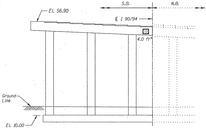
PIER 15 - SOUTH ELEVATION (Looking North)
