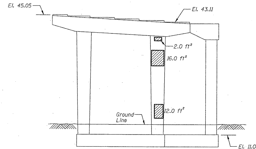
PIER H12 - ELEVATION (Looking East)
