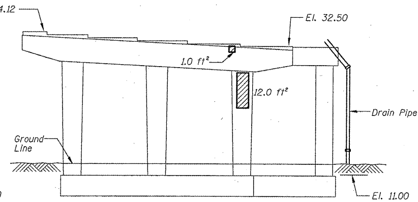
PIER H7 - ELEVATION (Looking East)
