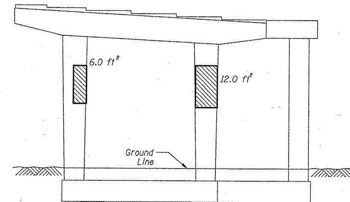
PIER H9 - ELEVATION (Looking East)
