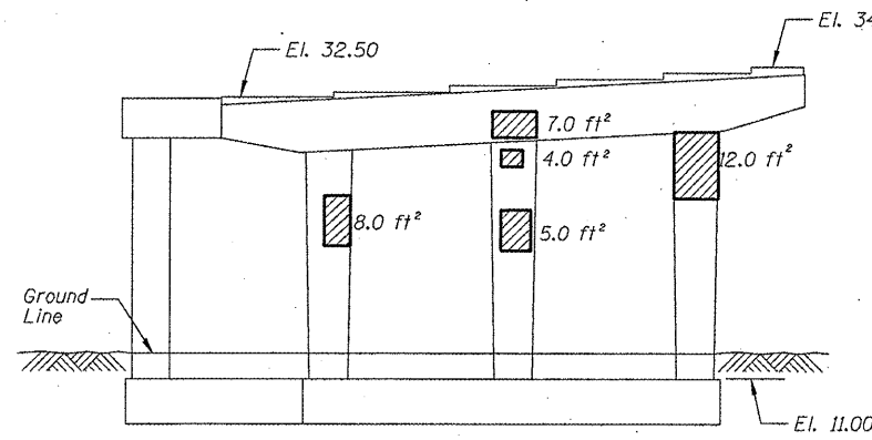
PIER H7 - ELEVATION (Looking West)
