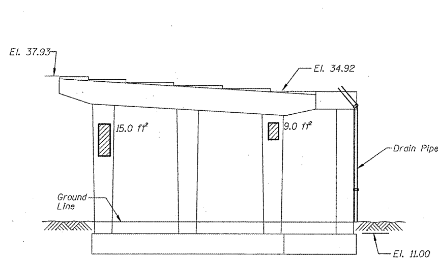
PIER H8 - ELEVATION (Looking East)
