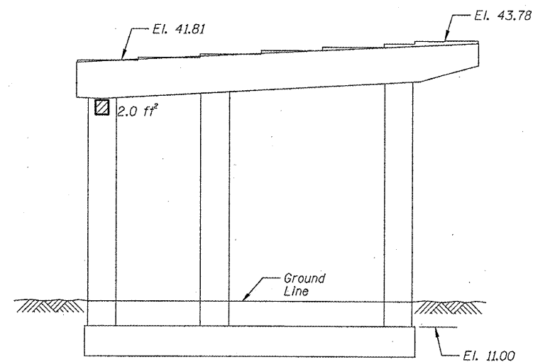
PIER H11 - ELEVATION (Looking West)
