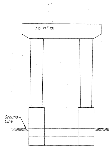
PIER 52 - WEST ELEVATION (Looking East)
