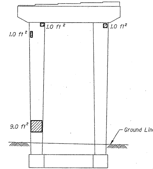
PIER 51 - EAST ELEVATION (Looking West)
