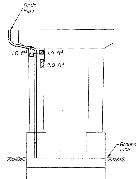
PIER 52 - EAST ELEVATION (Looking West)
