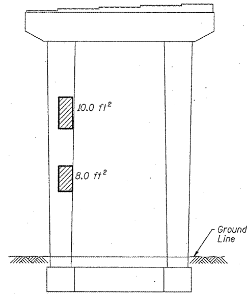
PIER 53 - EAST ELEVATION (Looking West)
