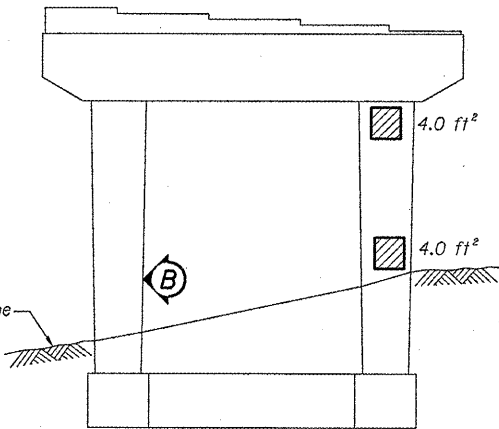
PIER 34 - NORTH ELEVATION (Looking South)
