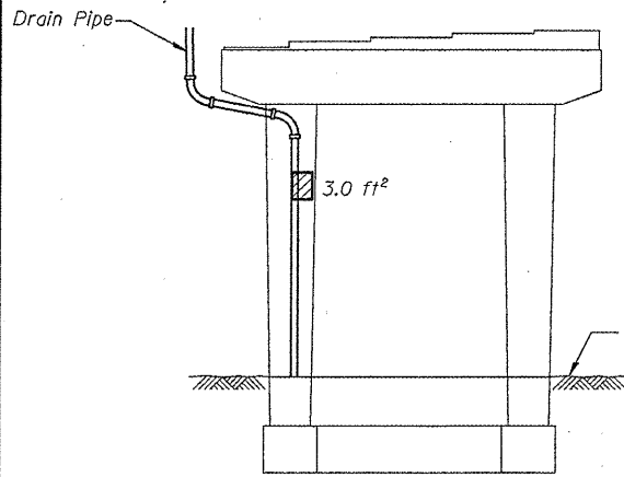
PIER 33 - SOUTH ELEVATION (Looking North)
