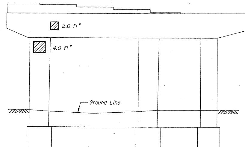
PIER 40 - NORTH ELEVATION (Looking South)
