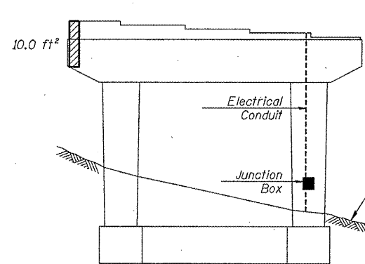
PIER 35 - NORTH ELEVATION (Looking South)
