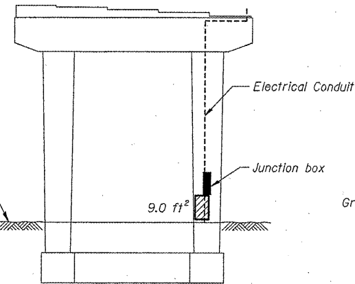
PIER 33 - NORTH ELEVATION (Looking South)
