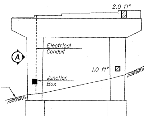
PIER 35 - SOUTH ELEVATION (Looking North)
