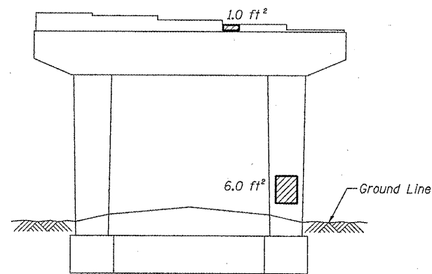
PIER 36 - NORTH ELEVATION (Looking South)
