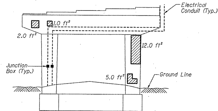
PIER 37 - NORTH ELEVATION (Looking South)
