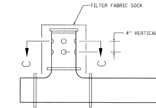
DETAIL A PERFORATED STAND PIPE PLAN
