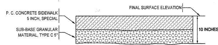
P.C. CONCRETE SIDEWALK 5 INCH, SPECIAL
