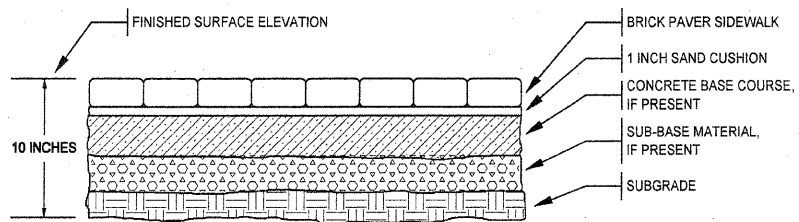
BRICK PAVER SIDEWALK REMOVAL
