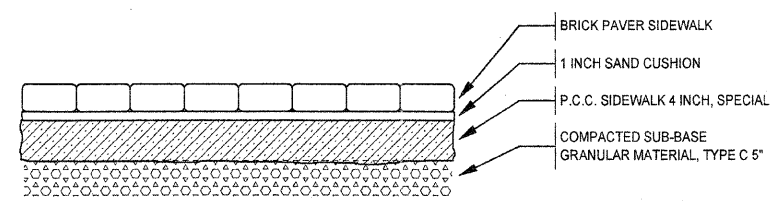
BRICK PAVER SIDEWALK REMOVAL AND REPLACEMENT
