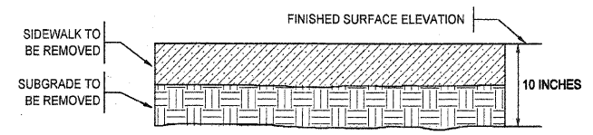
SIDEWALK REMOVAL, SPECIAL
