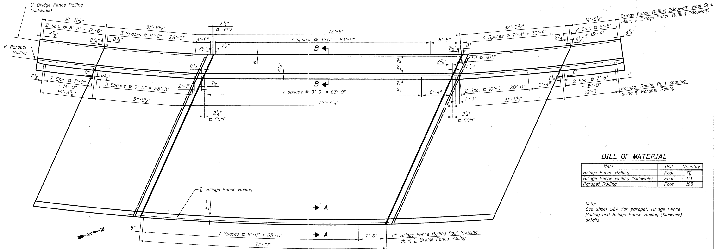
PLAN - PARAPET AND BRIDGE FENCE RAILING POST SPACING
