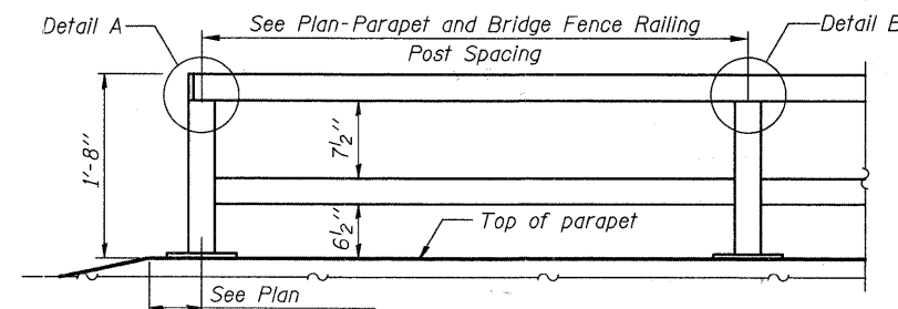
PARAPET RAILING - ELEVATION (Inside Face of Rail)
