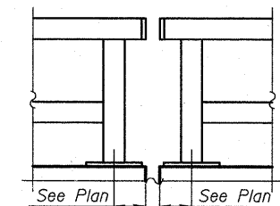
PARAPET RAILING ELEVATION AT EXPANSION JOINT
