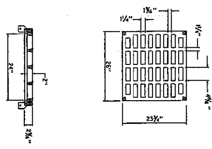
FRAME & GRATE DETAILS
