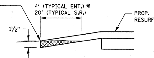
DETAIL A
