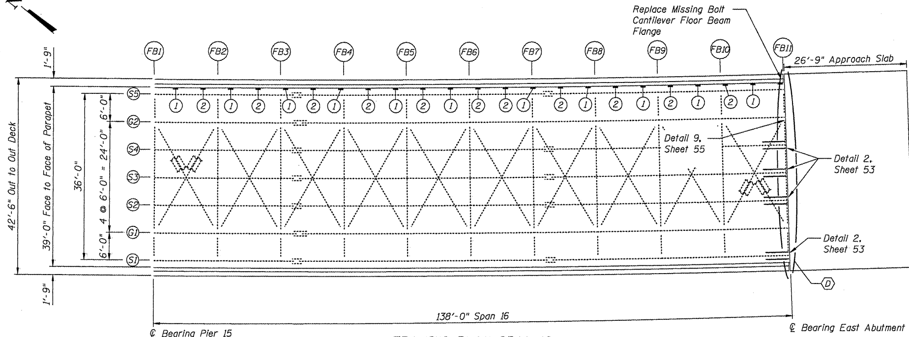
FRAMING PLAN SPAN 16 Westbound Lanes
