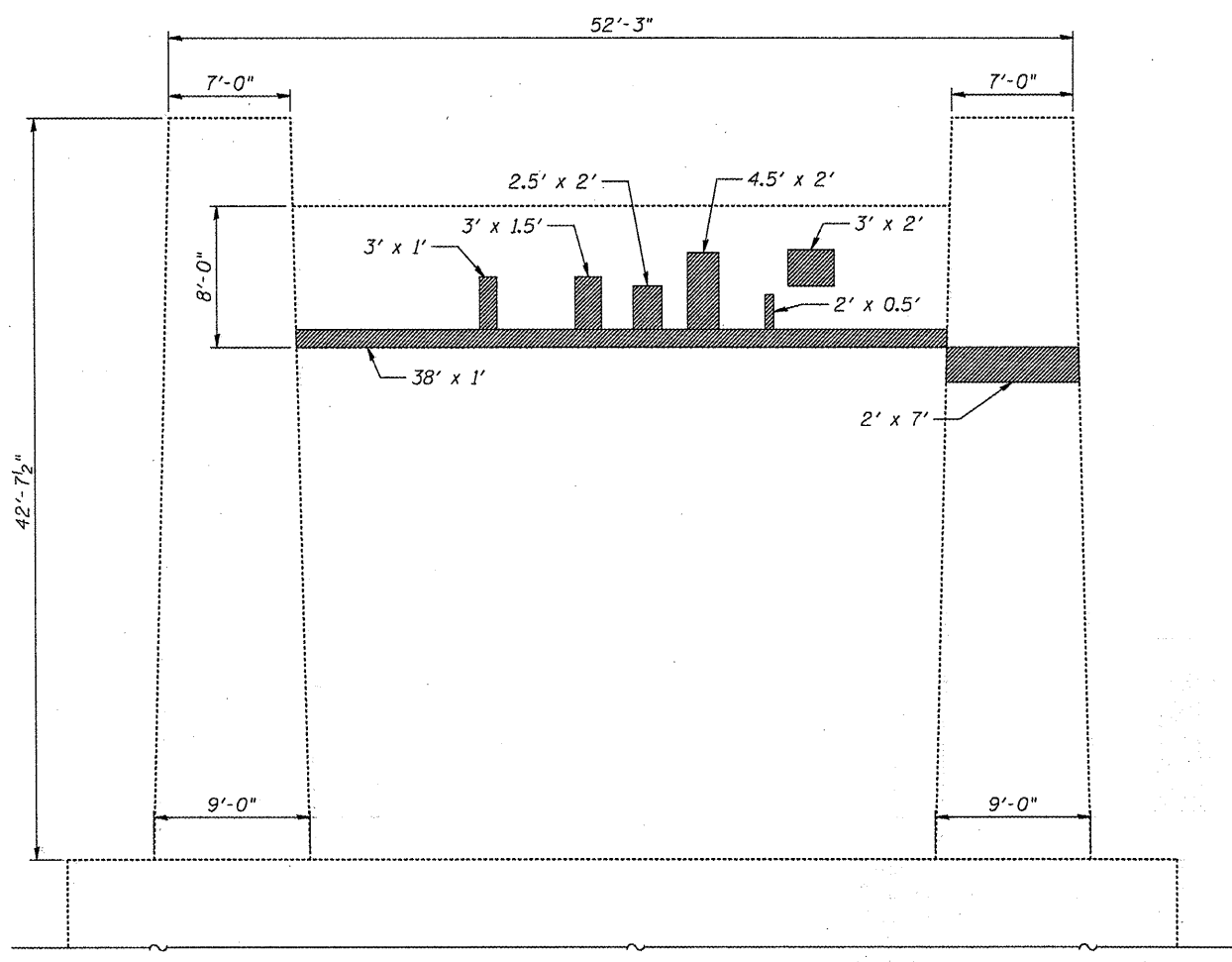
PIER 8 - EAST ELEVATION (Dimensions taken from existing drawings)
