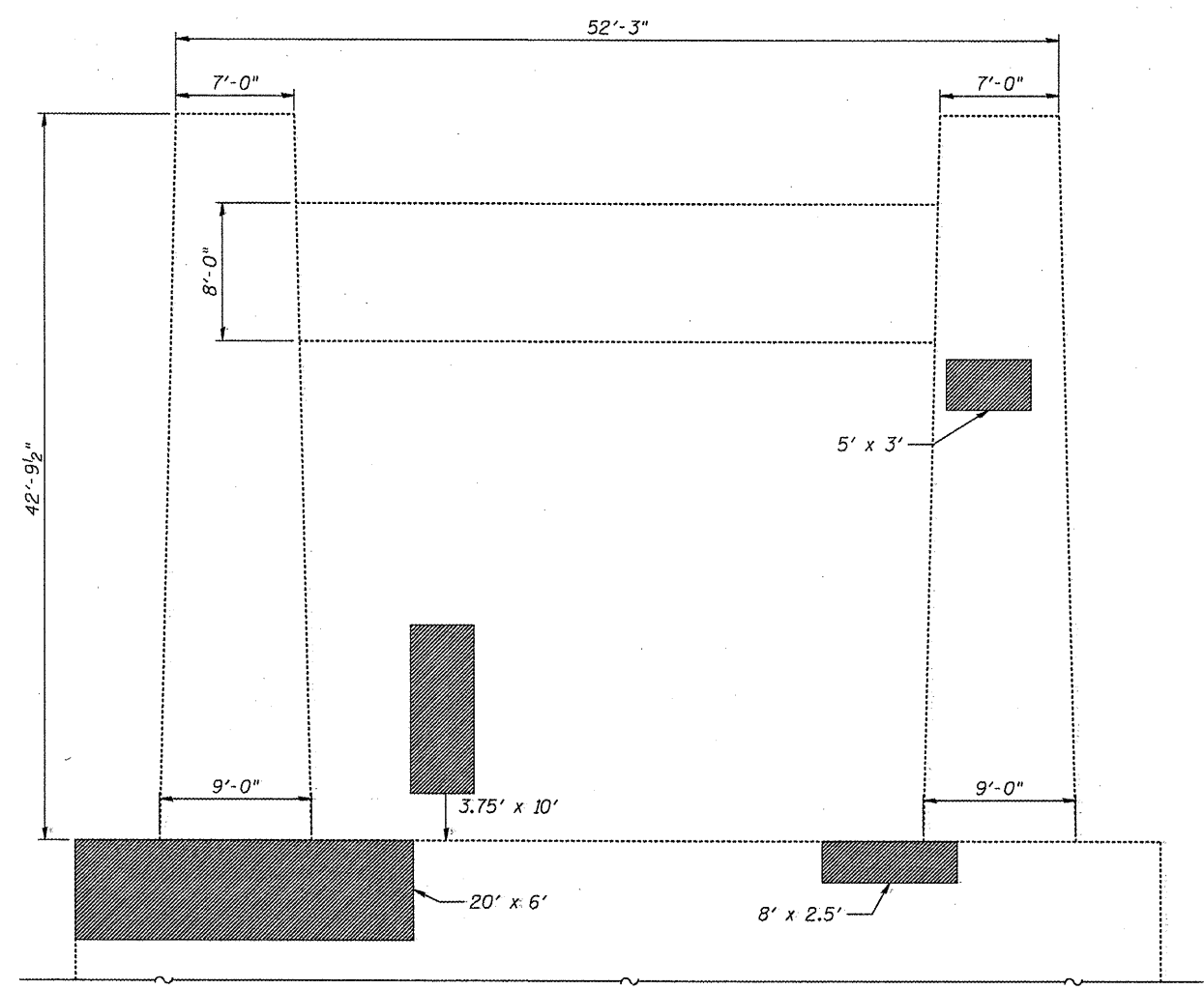
PIER 9 - WEST ELEVATION (Dimensions taken from existing drawings)
