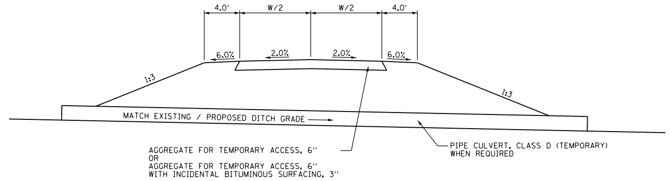
CROSS SECTION VIEW
