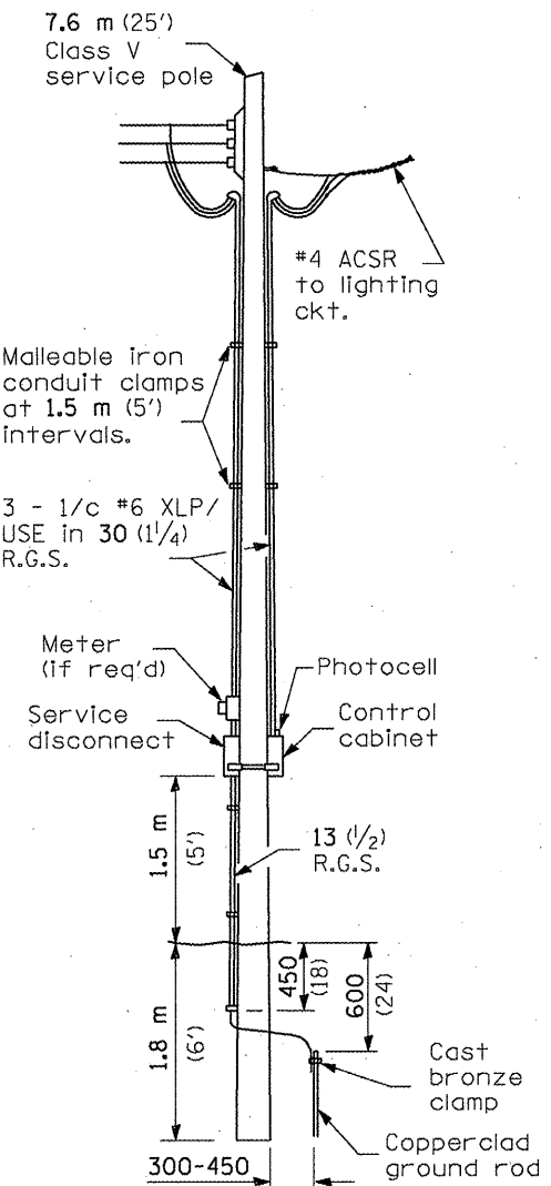
SERVICE INSTALLATION
