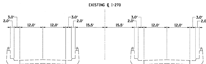
I-270 EXISTING MAINLINE WEST BRIDGE APPROACH SECTION STA 181+06 TO STA 191+50
