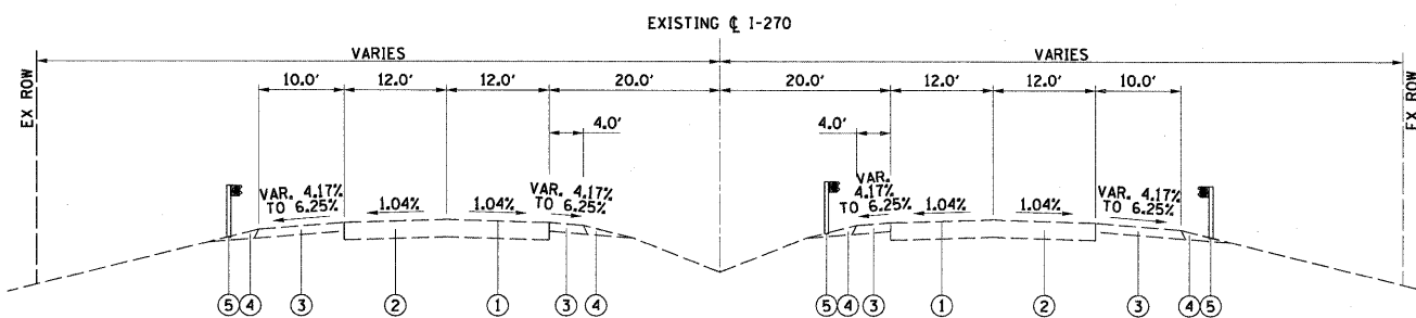
I-270 EXISTING MAINLINE WEST BRIDGE APPROACH SECTION STA 181+06 TO STA 191+50
