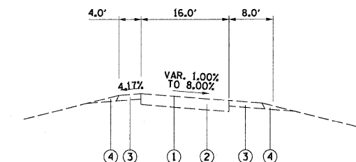
I-270 EXISTING EB RAMP FROM NB IL RT 3 RAMP E4
