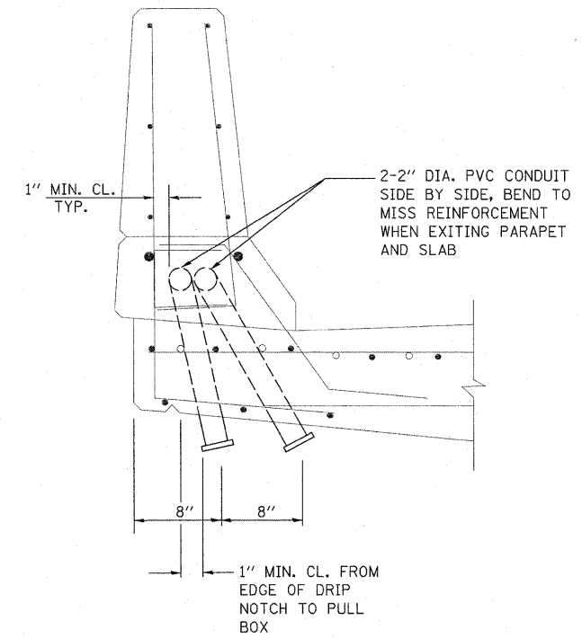
VIEW B-B
