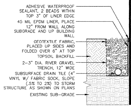
L 4-9 WATERPROOF LINER AND DRAIN TILE NOT TO SCALE
