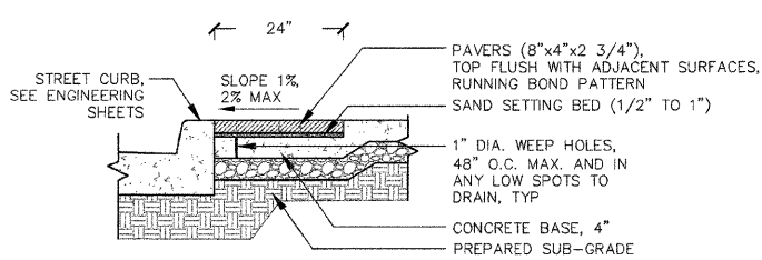
L 4-2 BRICK PAVER BORDER ADJACENT TO CURB/SIDEWALK NOT TO SCALE
