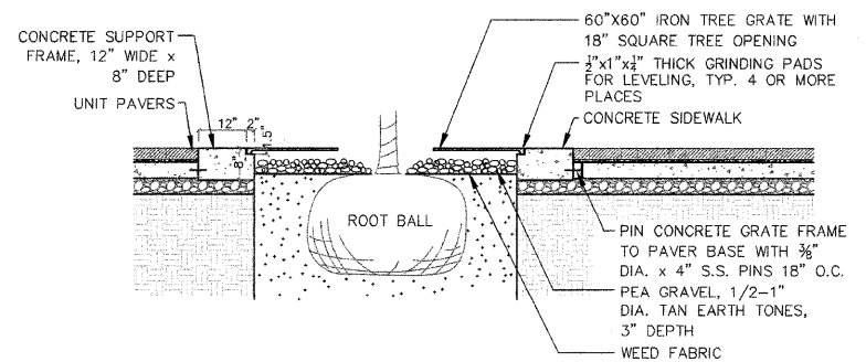
L 4-5 TREE GRATE IN PLAZA AREA NOT TO SCALE
