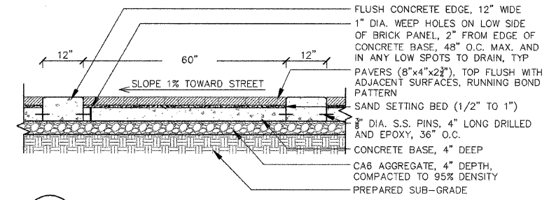
L 4-3 BRICK PAVERS AND FLUSH CONCRETE CURBS NOT TO SCALE
