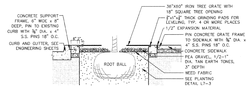
L 4-4 TREE GRATE ADJACENT TO CURB AND SIDEWALK NOT TO SCALE
