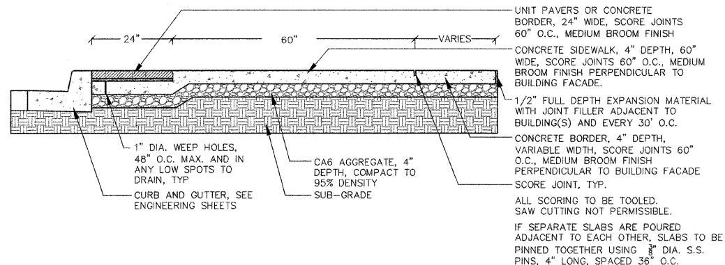
L 4-1 CONCRETE SIDEWALK AND BORDERS NOT TO SCALE
