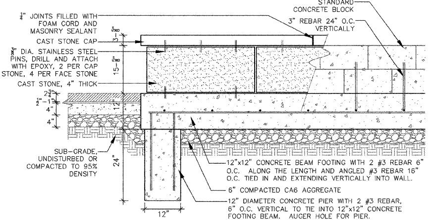
L 4-7 STONE RETAINING WALL NOT TO SCALE
