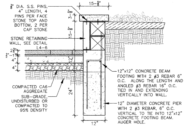
L 4-8 STONE RETAINING WALL NOT TO SCALE
