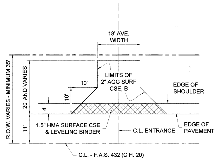
ENTRANCE DETAIL
