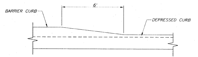
DETAIL OF CURB HEIGHT TRANSITION (DETAIL "A")
