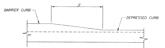
DETAIL OF CURB HEIGHT TRANSITION (DETAIL "B")
