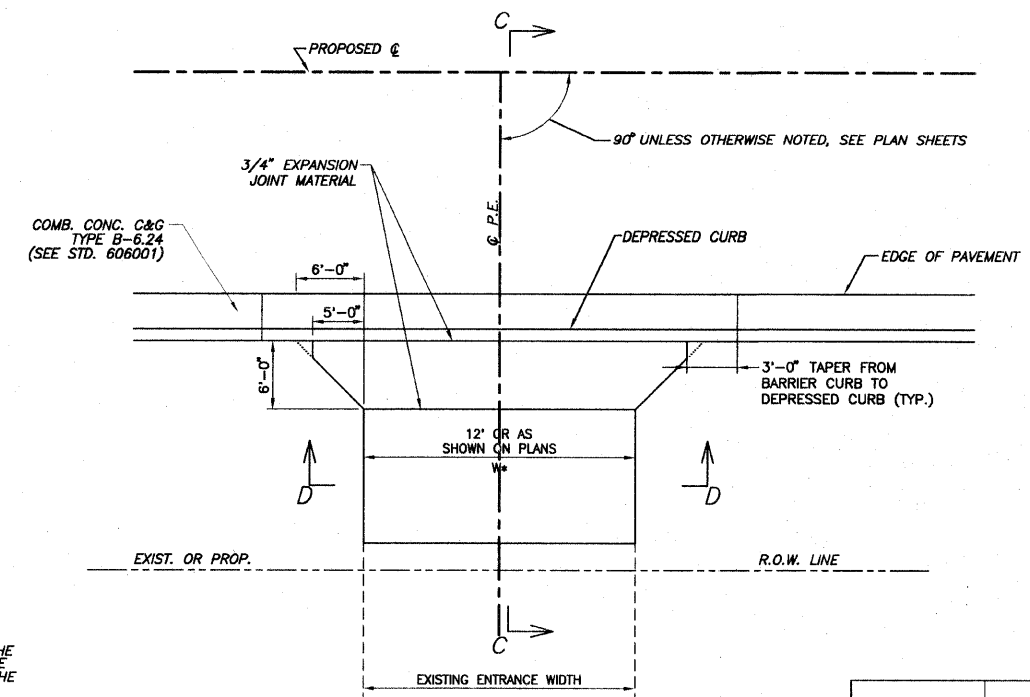
P.E. DETAIL "B" PRIVATE ENTRANCE WITHOUT SIDEWALK N.T.S.
