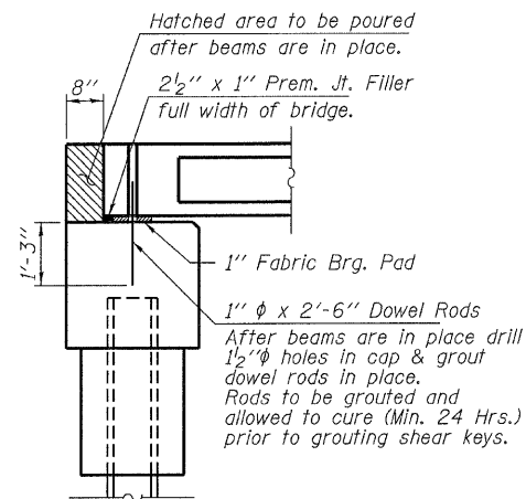
SECTION AT ABUTMENTS © R.I. L's
