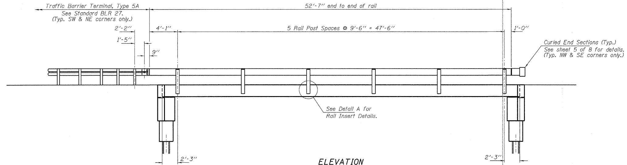
ELEVATION Showing Rail Post Spacing See sheet 5 of 8 for Railing Details.
