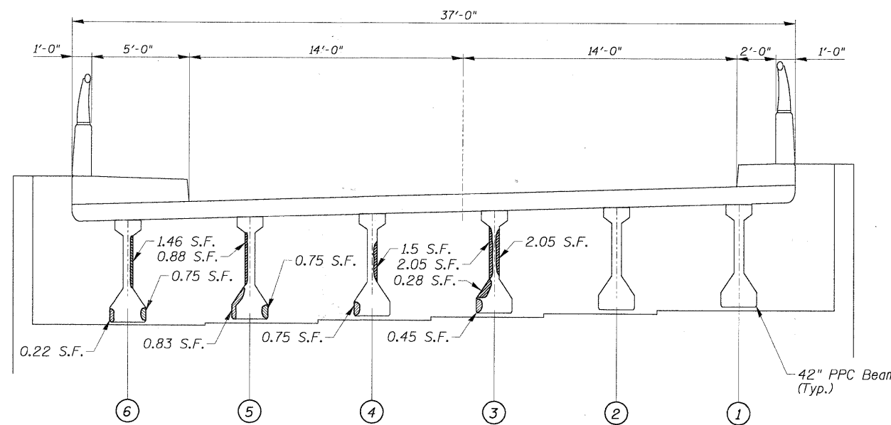
SOUTH ABUTMENT
