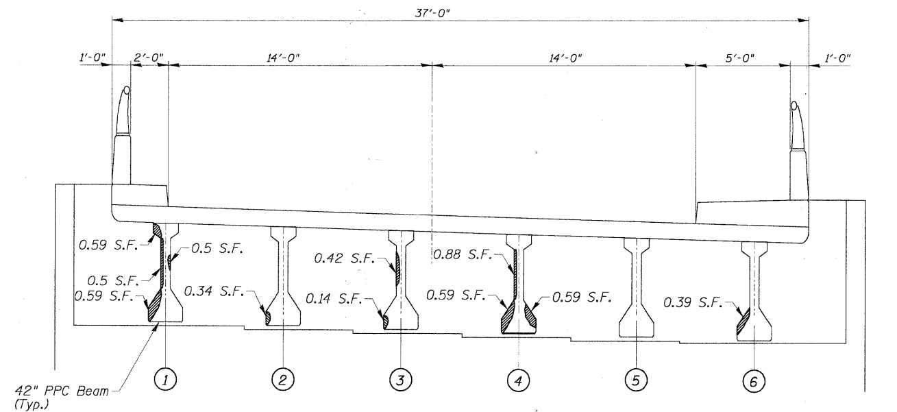
NORTH ABUTMENT
