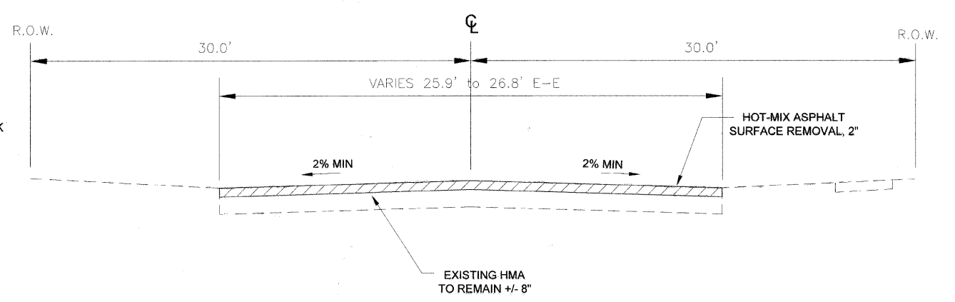
EXISTING TYPICAL SECTION STA. 8+19.19 to STA. 30+89.16, HARWOOD AVENUE
