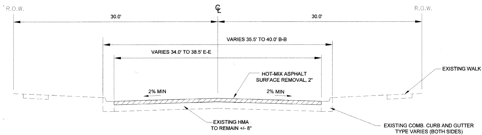
EXISTING TYPICAL SECTION STA. 0+00 to STA. 2+41.93, HARWOOD AVENUE
