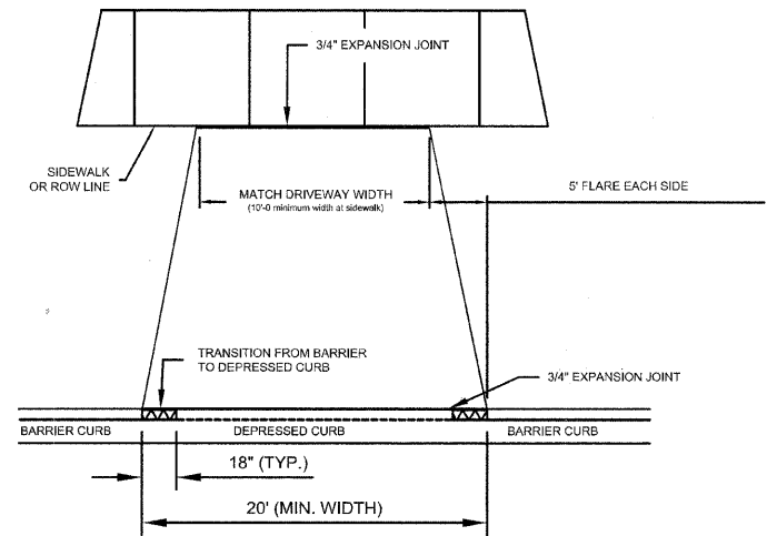
TYPICAL DRIVEWAY DETAIL
