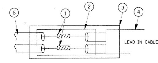
PRE-FORMED LOOP
