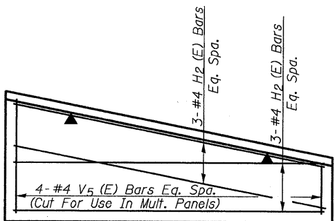
PANEL D REINFORCEMENT
