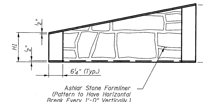
TYPICAL PANEL ELEVATION
