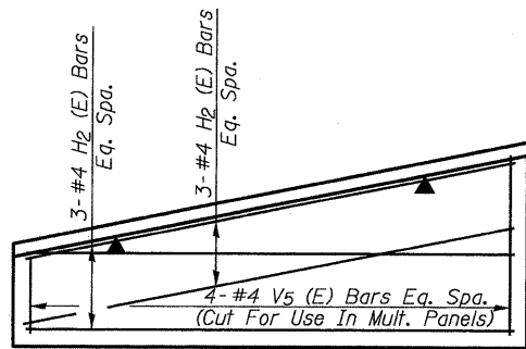
PANEL B REINFORCEMENT
