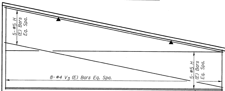
PANEL I REINFORCEMENT
