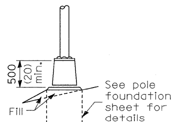
TRANSFORMER BASE
