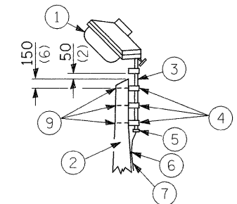
TENON
