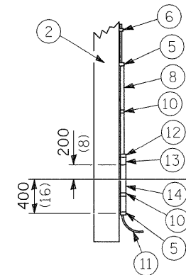
POLE, WOOD
