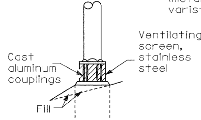
BREAKAWAY COUPLING
