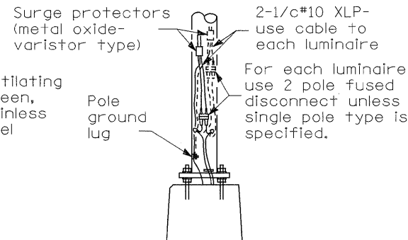
ANCHOR
