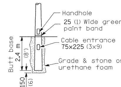
BUTT BASE
