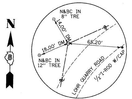
QUARRY ROAD PI STA 56+66.90 N - 849631.87 E - 2277512.81 5/8" I. ROD W/CAP
