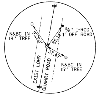
QUARRY ROAD POT STA 54+50 N - 849429.27 E - 2277435.37 RR SPIKE W/PUNCH HOLE BURIED 4"
