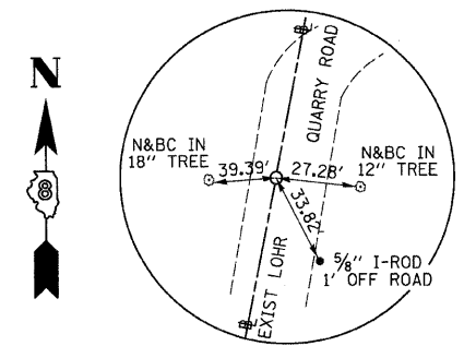
QUARRY ROAD PC STA 55+64.05 N - 849535.79 E - 2277476.09 RR SPIKE W/PUNCH HOLE BURIED 4"
