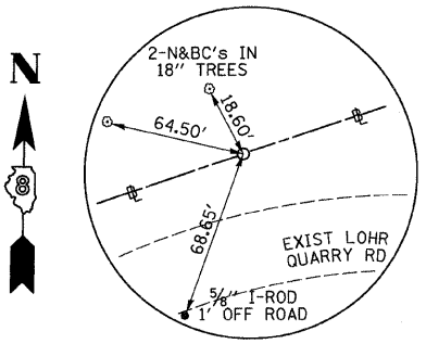
QUARRY ROAD PC STA 58+26.04 N - 849718.29 E - 2277655.33 5/8" I. ROD W/CAP
