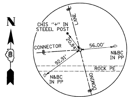
CONNECTOR ROAD POT STA 53+60 N - 850956.27 E - 2277748.51 5/8" I. ROD W/CAP
