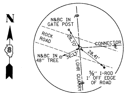
CONNECTOR ROAD POT STA 50+00 N - 850812.50 E - 2277418.47 RR SPIKE W/PUNCHHOLE BURIED 4"
