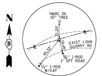
QUARRY ROAD PT STA 57+62.22 N - 849685.20 E - 2277600.77 RR SPIKE W/PUNCH HOLE BURIED 3"
