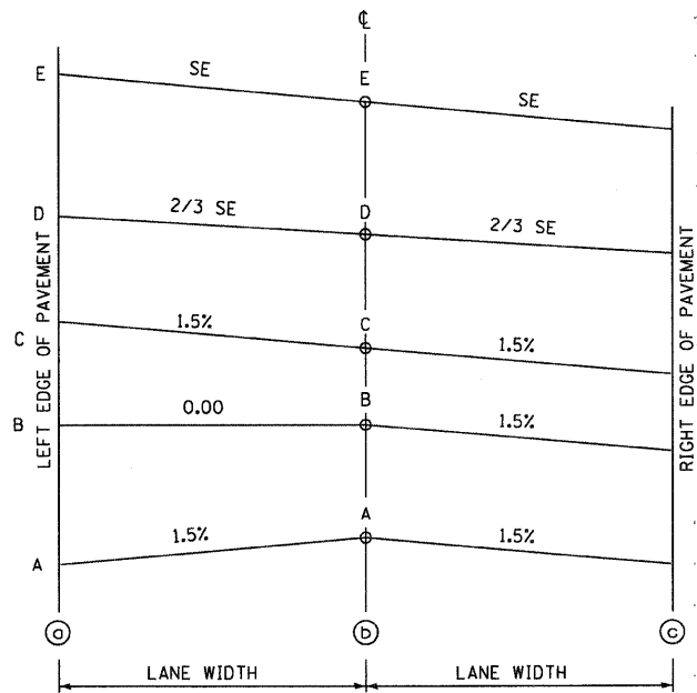
TYPICAL CROSS SECTION - SE TRANSITION
