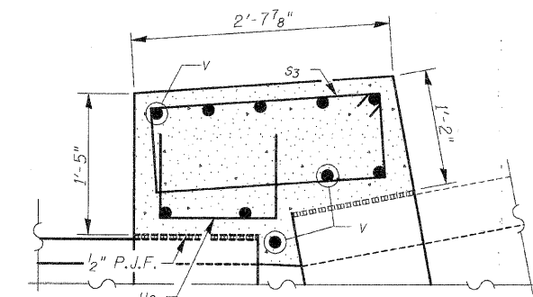
SECTION THRU WEST SIDEWALL
