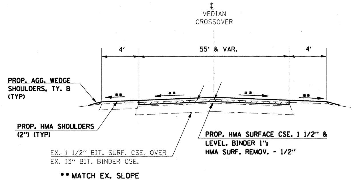
SECTION D - D TYPICAL FOR MEDIAN CROSSOVER
