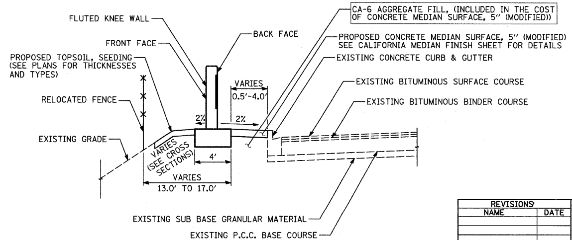
KNEE WALL DETAIL 4
