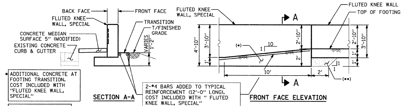
FOOTING TRANSITION - DETAIL 1 (FROM FLUTED KNEE WALL, SPECIAL TO FLUTED KNEE WALL)
