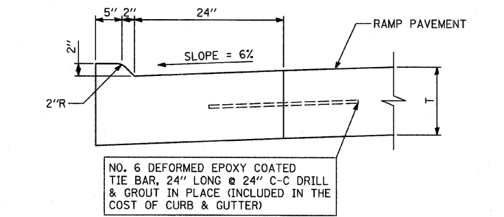
COMBINATION CONCRETE CURB & GUTTER, TYPE M-2.24
