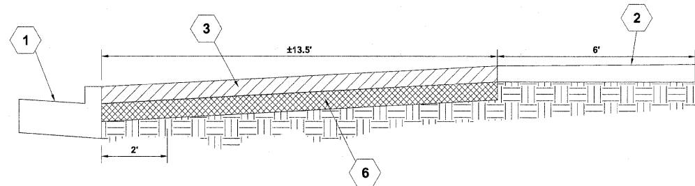
EXISTING TYPICAL CROSS SECTION SOUTH SIDE OF ROOSEVELT ROAD (STA. 327+44 TO STA. 327+64)
