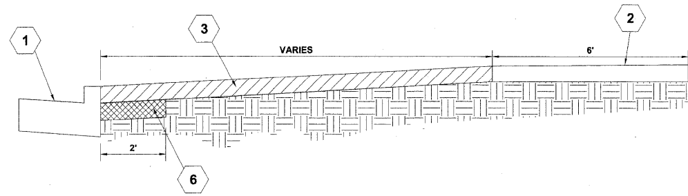
EXISTING TYPICAL CROSS SECTION SOUTH SIDE OF ROOSEVELT ROAD (STA. 326+07 TO STA. 326+33)
