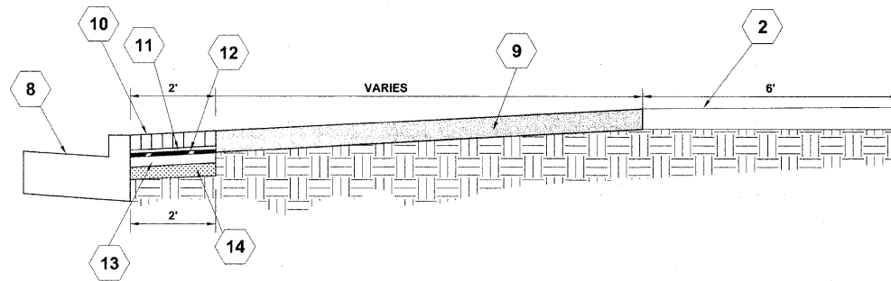
PROPOSED TYPICAL CROSS SECTION SOUTH SIDE OF ROOSEVELT ROAD (STA. 326+07 TO STA. 326+33)
