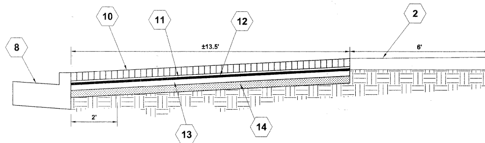
PROPOSED TYPICAL CROSS SECTION SOUTH SIDE OF ROOSEVELT ROAD (STA. 327+44 TO STA. 327+64)
