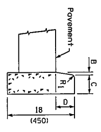
BARRIER CURB
