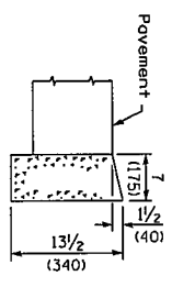
DEPRESSED CURB
