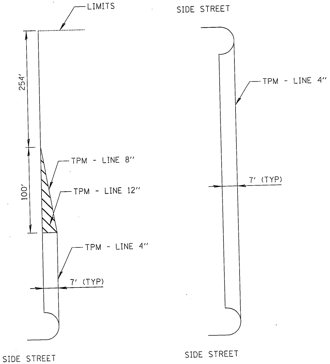
PAVEMENT STRIPING BETWEEN SIDE STREET ENTRANCES (TYP)
