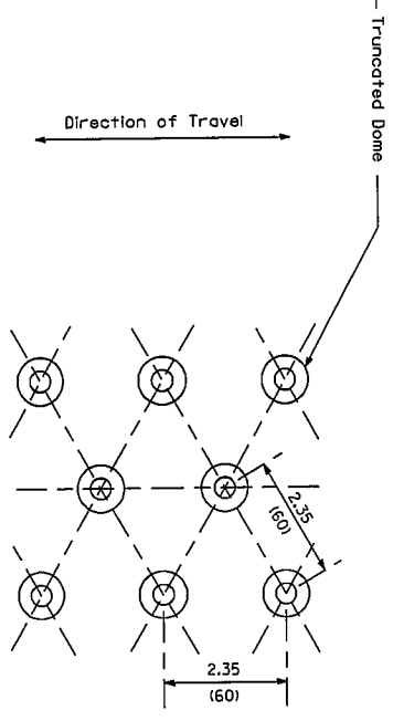
TRIANGULAR PATTERN
