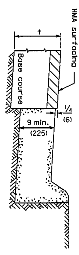
ON UNDISTURBED SUBGRADE
