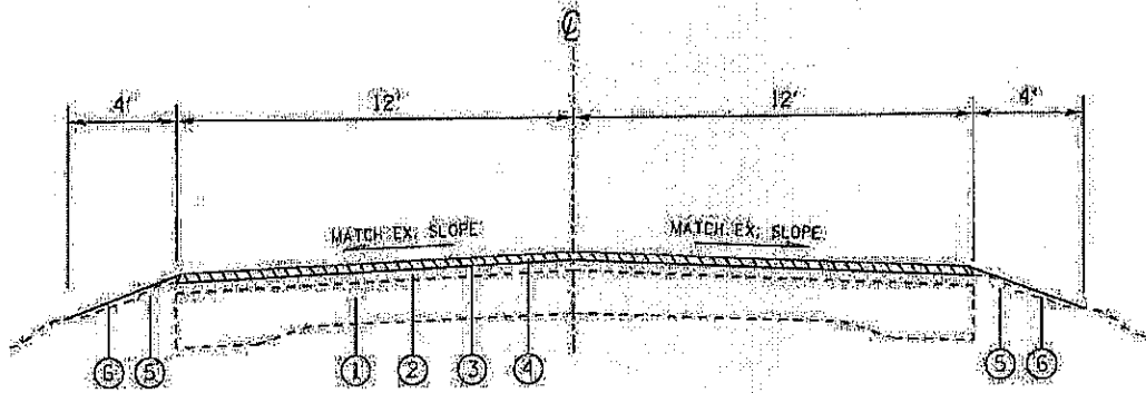
TYPICAL SECTION STA. 0+00 TO 11+00 SHILOH RD.
