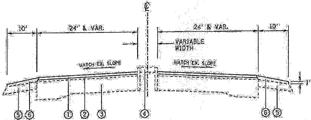
TYPICAL SECTION STA 17+70 TO 38+13 IL RTE 111
